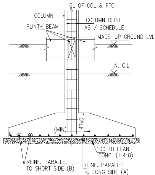
(A = LONG SIDE, B = SHORT SIDE) TYP. SECTION OF ISOLATED FOOTING. (F1 )
