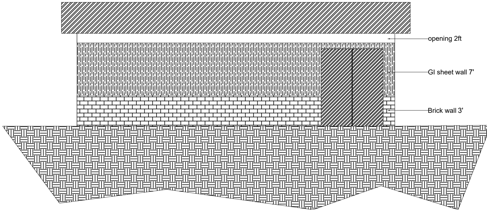
SIDE ELEVATION
