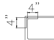
SECTION (AT COL-BEAM JUNCTION)
