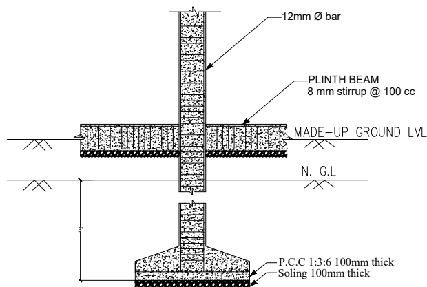
FOOTING SECTION
