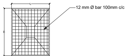
BRIDGE PLAN
